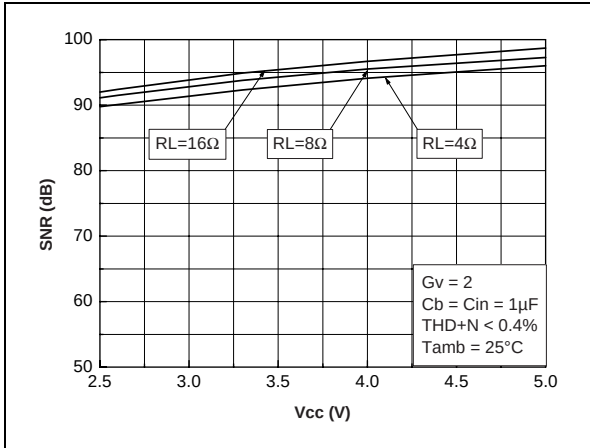
Fig. 69 : Signal to Noise Ratio vs Power Supply with Unweighted Filter (20Hz to 20kHz)
