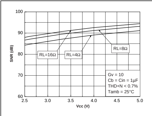
Fig. 70 : Signal to Noise Ratio vs Power Supply with Weighted Filter Type A
